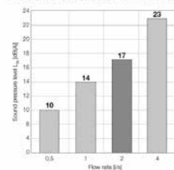
Sound pressure levels L_N of the PP3 pipe in compliance with DIN 4109
